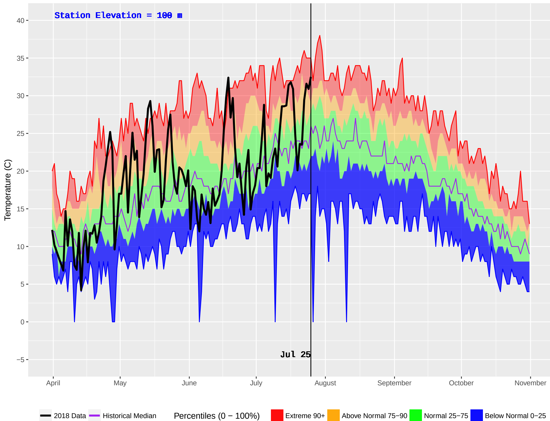
BEAVER CREEK (37) : Historical (1987–2016) and Current (2018) Noon Temperature
