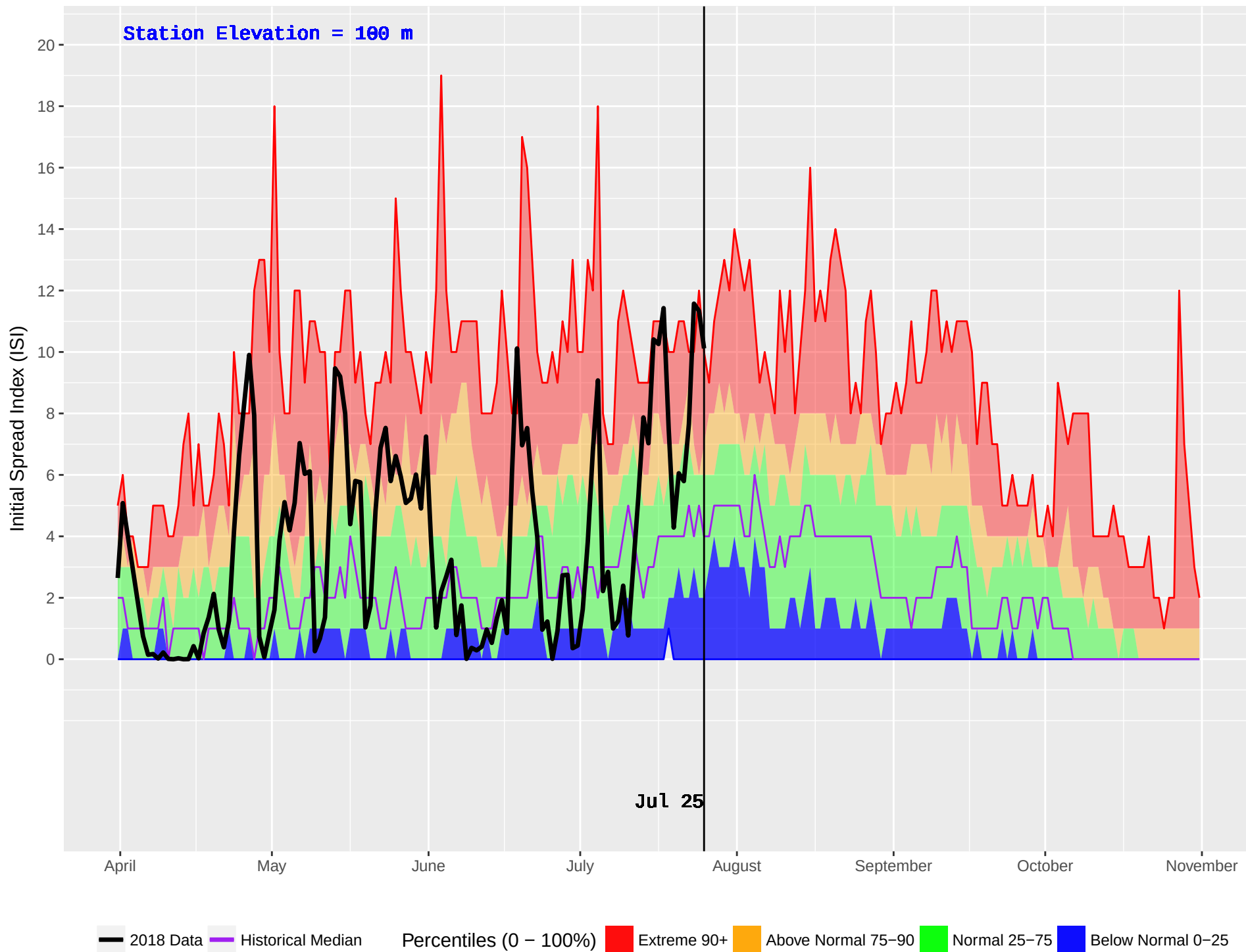
BEAVER CREEK (37) : Historical (1987–2016) and Current (2018) Noon Initial Spread Index (ISI)
