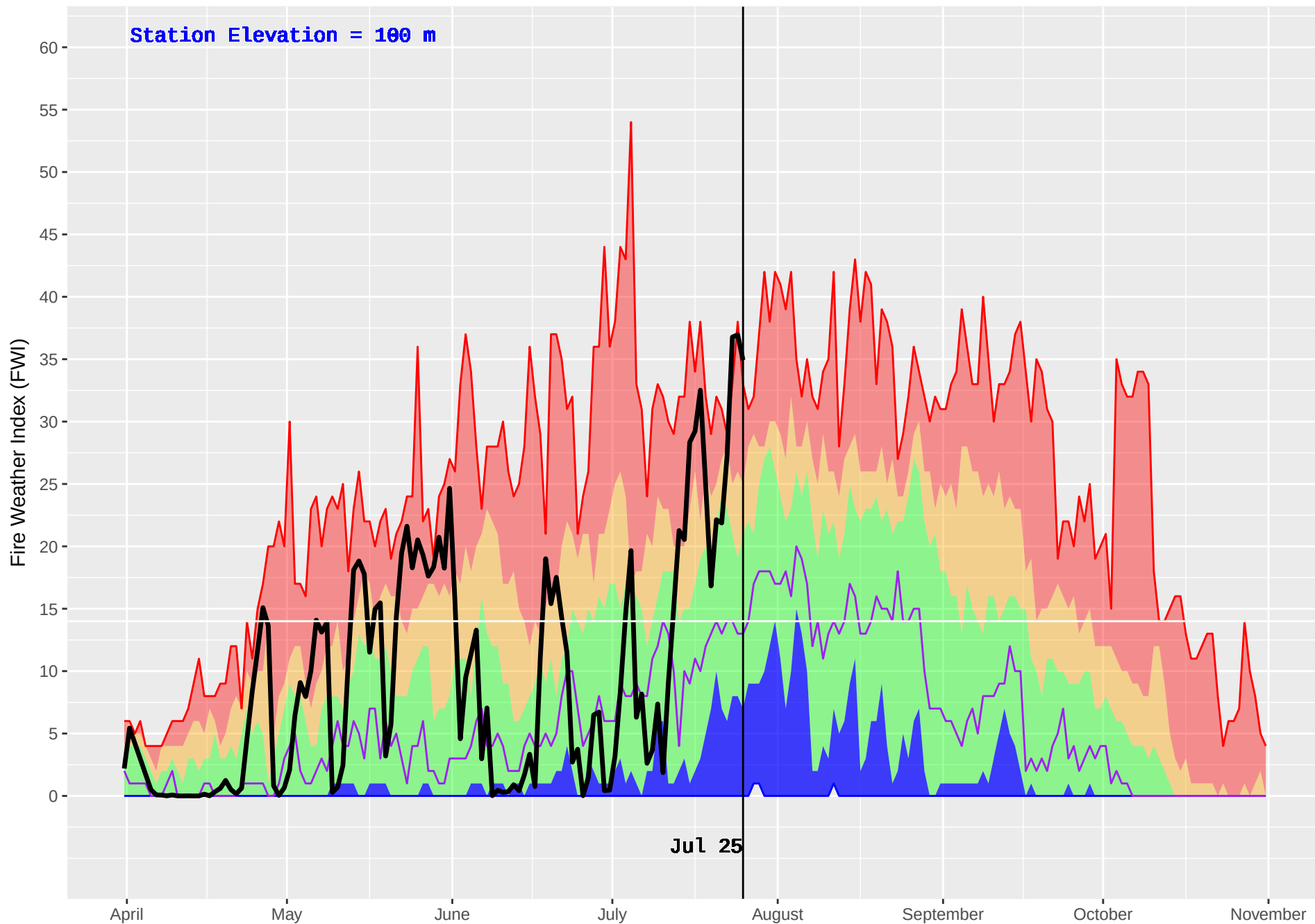
BEAVER CREEK (37) : Historical (1987–2016) and Current (2018) Noon Fire Weather Index (FWI)
