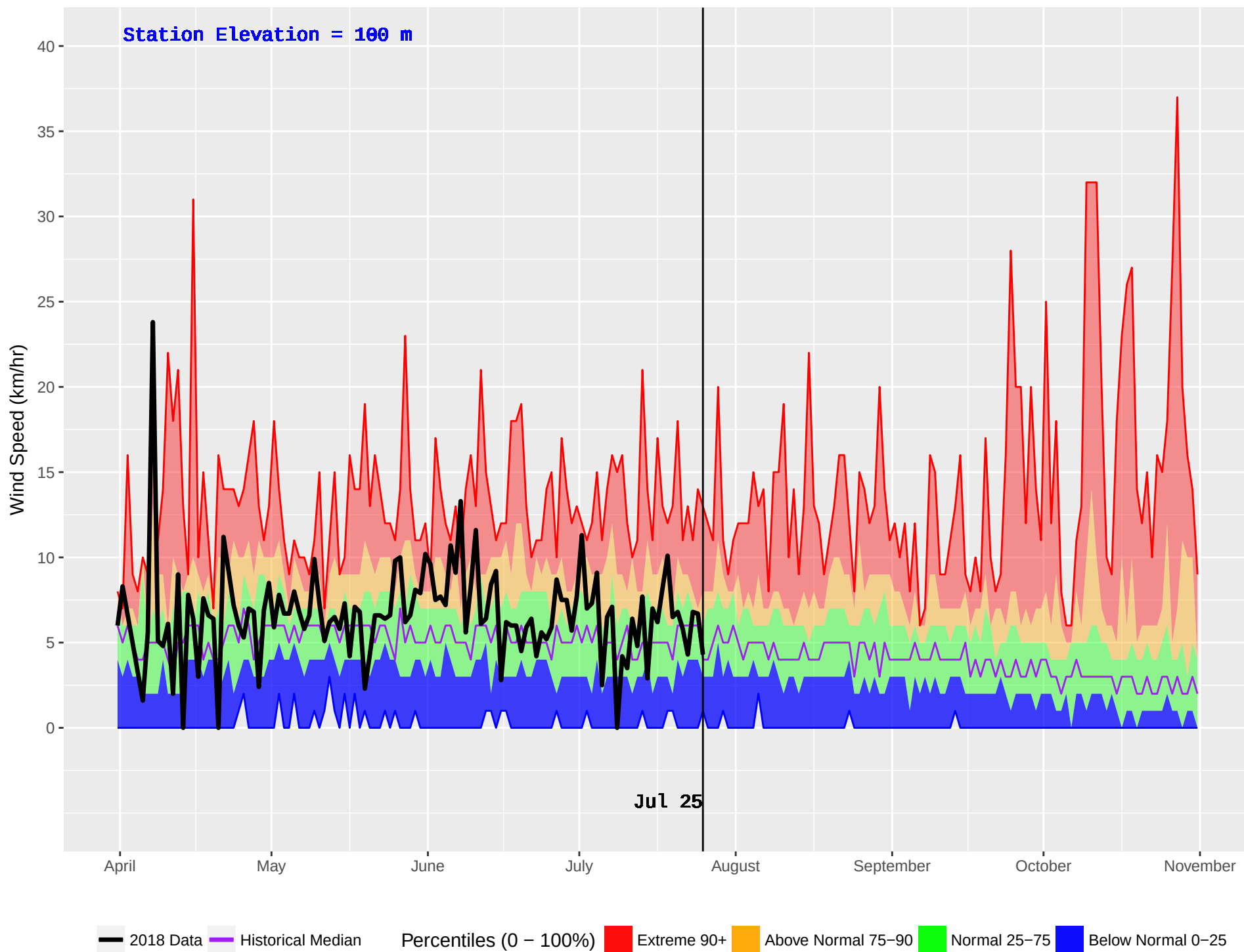
BEAVER CREEK (37) : Historical (1987–2016) and Current (2018) Noon Wind Speed
